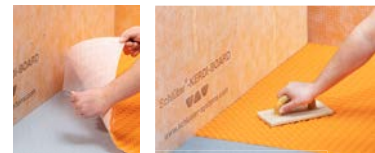
DITRA-HEAT-PS
